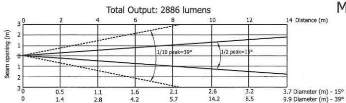
LEDWash300X Photometrics
