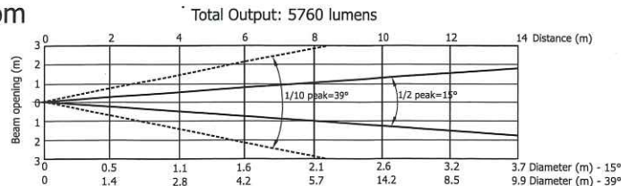
LEDWash600X Photometrics
